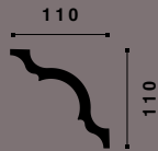
GT NOMASTYL®
