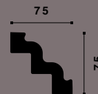
B1 NOMASTYL®
