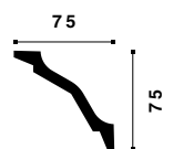
WT26 WALLSTYL® 75 x 75 x 2000mm
