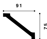
WT2 WALLSTYL® 75 x 91 x 2000 mm
