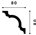
GO NOMASTYL® 80 x 80 x 2000 mm
