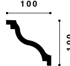
SL NOMASTYL® 100 x 100 x 2000 mm
