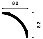
B8 NOMASTYL® 82 x 82 x 2000 mm
