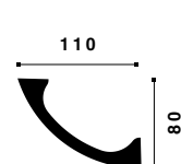
WT3 WALLSTYL®
